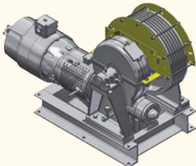
Traction Sheave Rope Retainer
